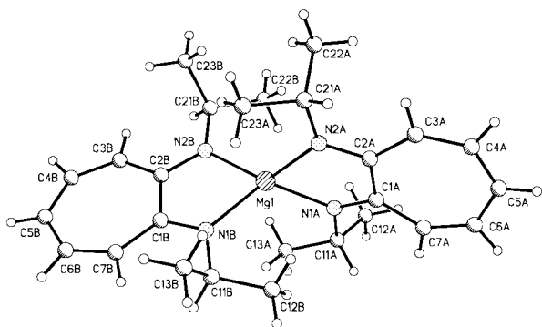
Fig. 4 Molecular structure of [\text{Mg}\{\eta^2\text{-}(\text{iPr}_2)\text{ATI}\}_2]_2 5 .
