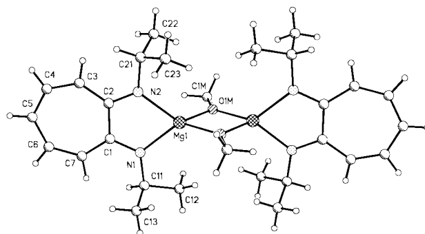
Fig. 2 Molecular structure of [\text{Mg}(\mu\text{-OMe})\{\eta^2\text{-}(\text{Pr}_2)\text{ATI}\}_2] 3 .
